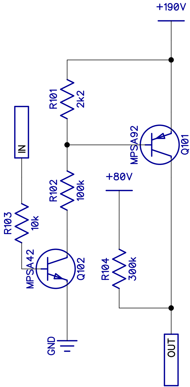
Anode driver
