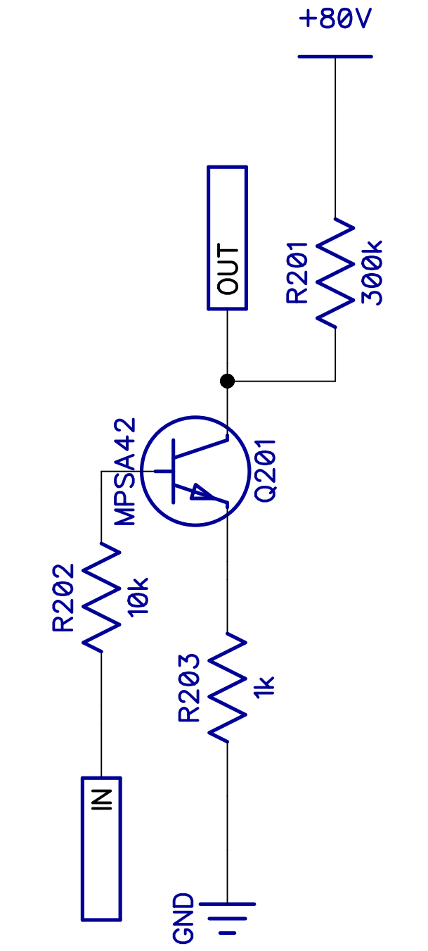
Cathode driver
